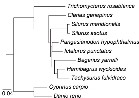
c Fish dataset topologies
