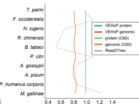
f Insects dataset root-to-tip distance
