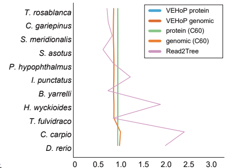
d Fish dataset root-to-tip distance
